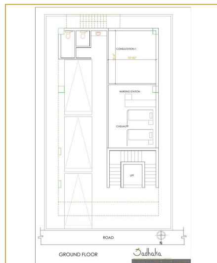
AOI Hospital, Nakkal Road — ground floor
